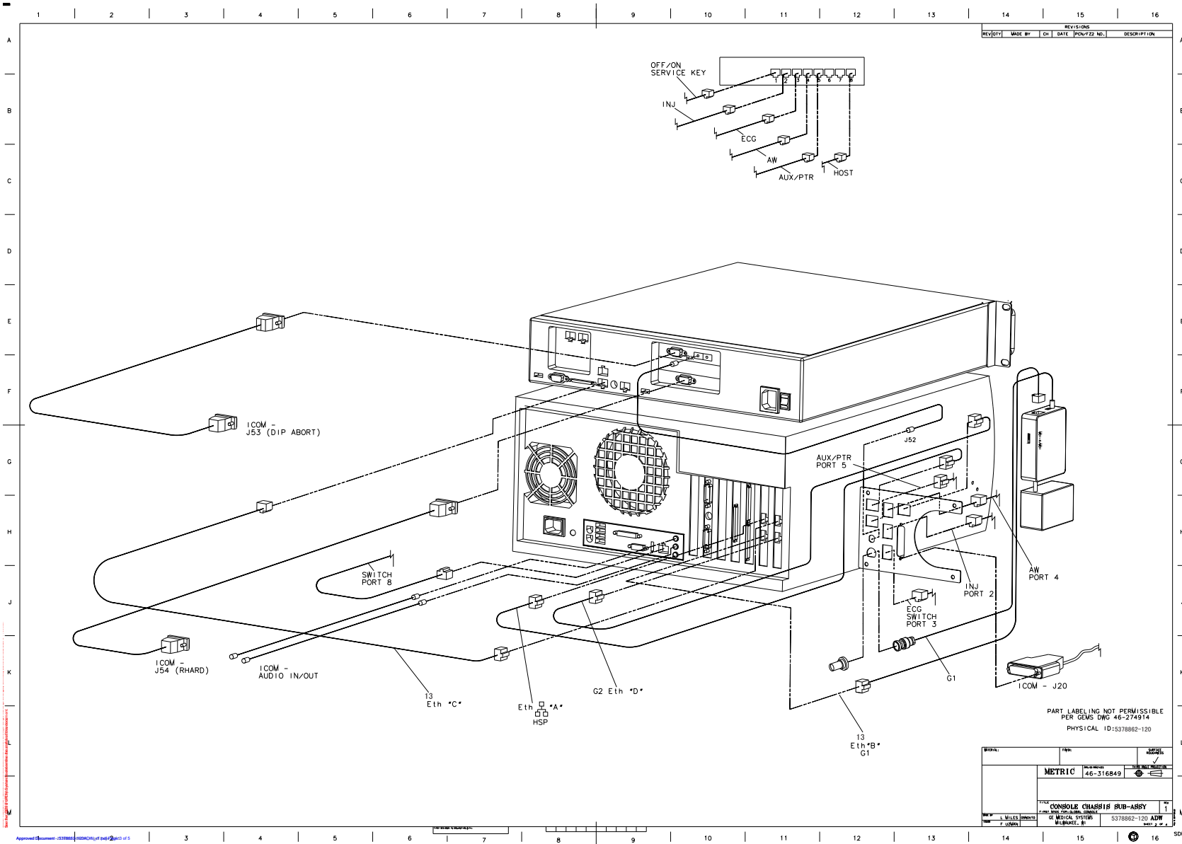
Figure 5-2 LCGOC Freedom Workspace (5378862-120 Sheet 2, Rev 1)
