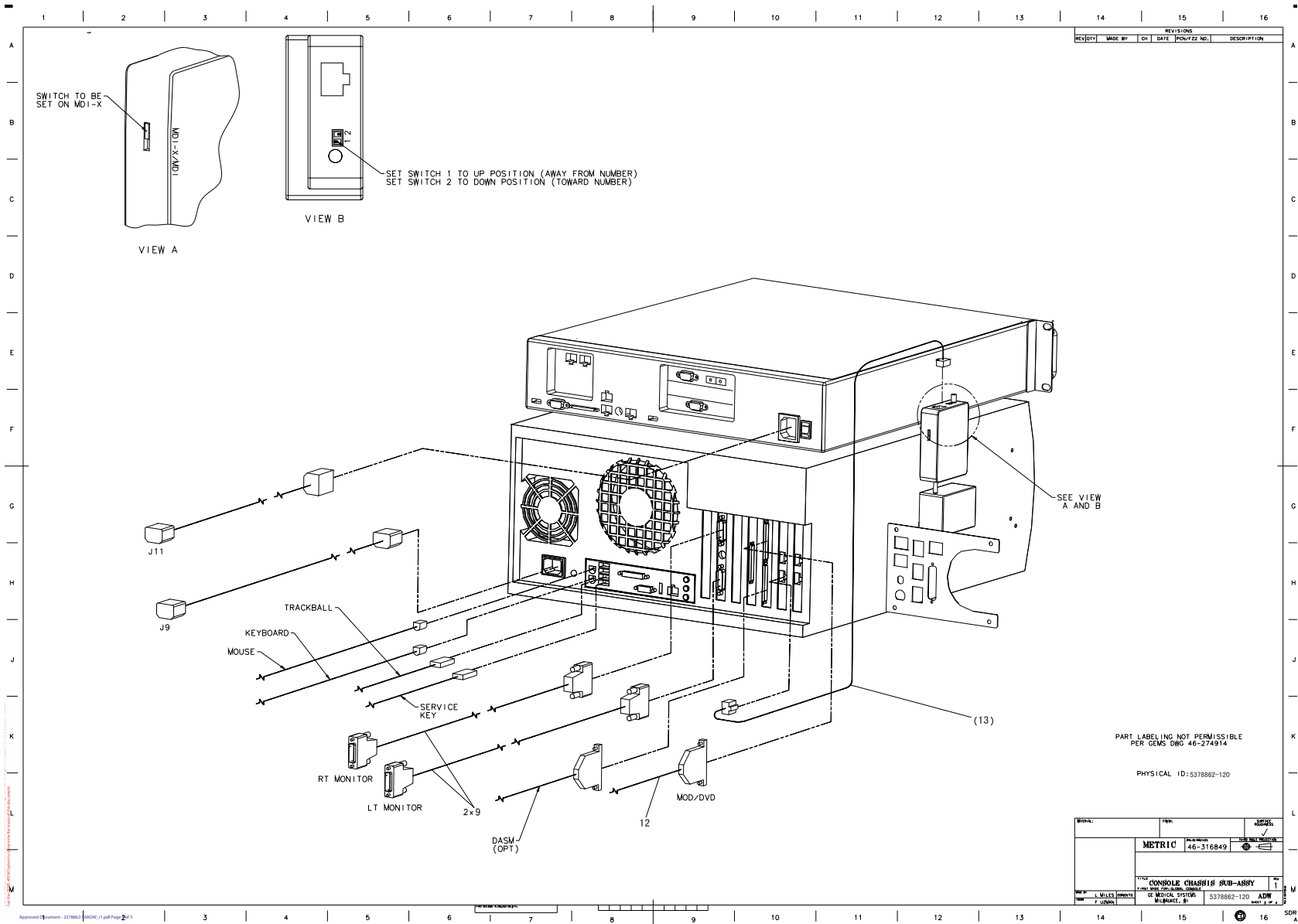
Figure 5-3 LCGOC Freedom Workspace (5378862-120 Sheet 3, Rev 1)
