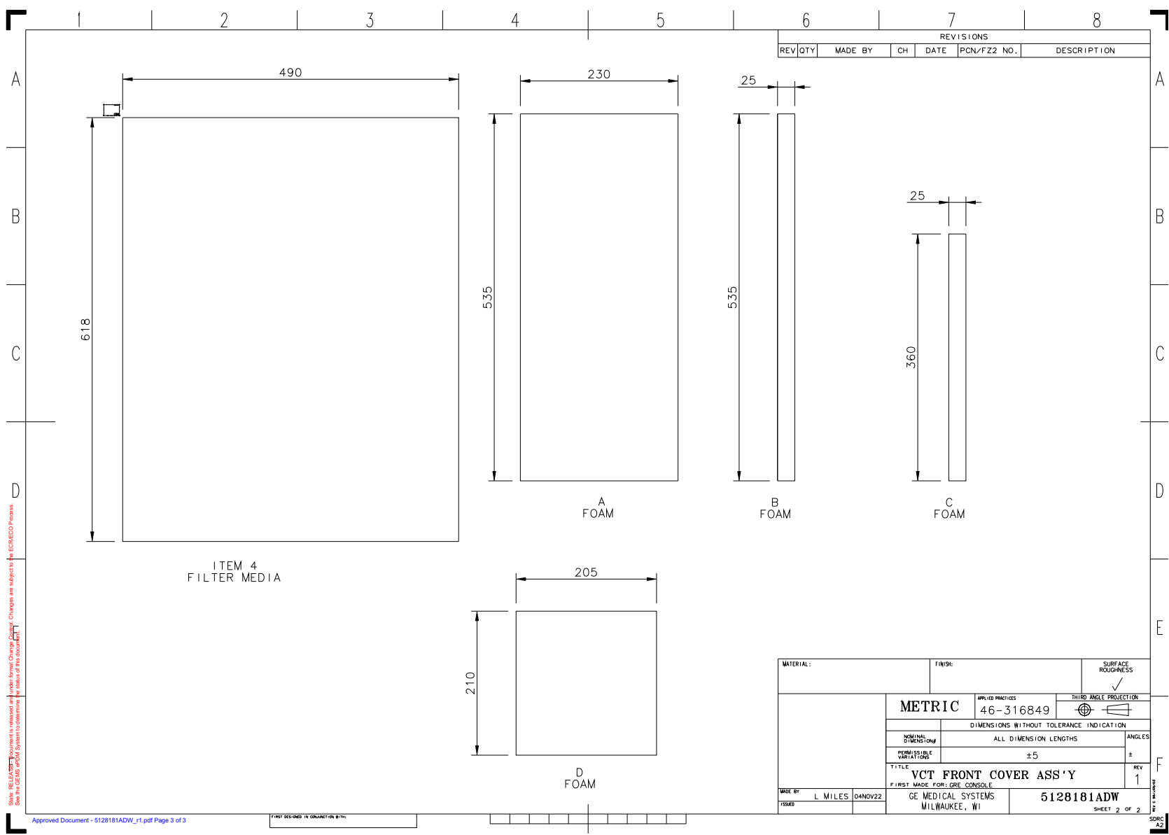
Figure 5-19 Cover Assy - Console Front (5128181 Sheet 2, Rev 1)
