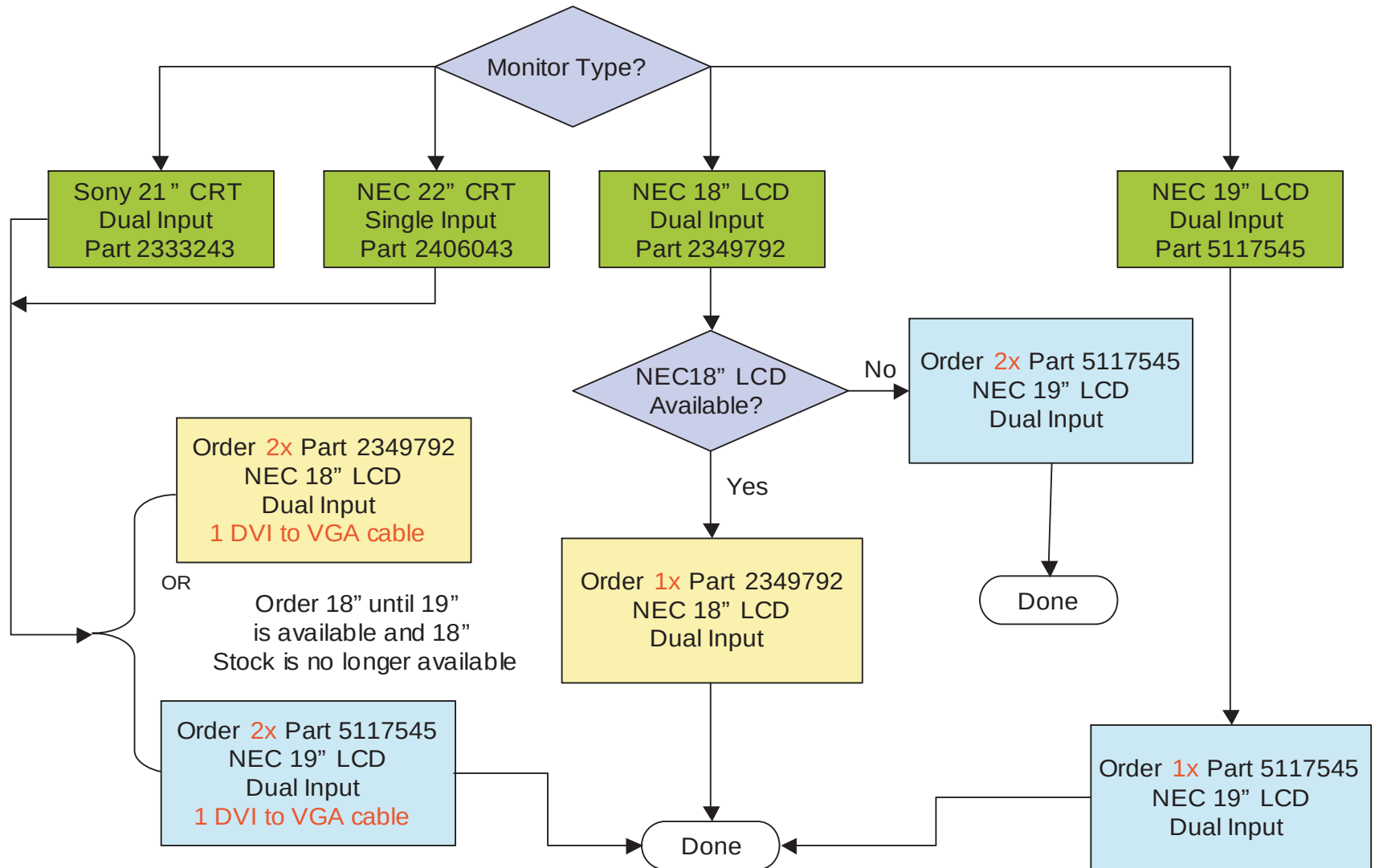
Figure 5-10 Monitor Selection Flowchart
