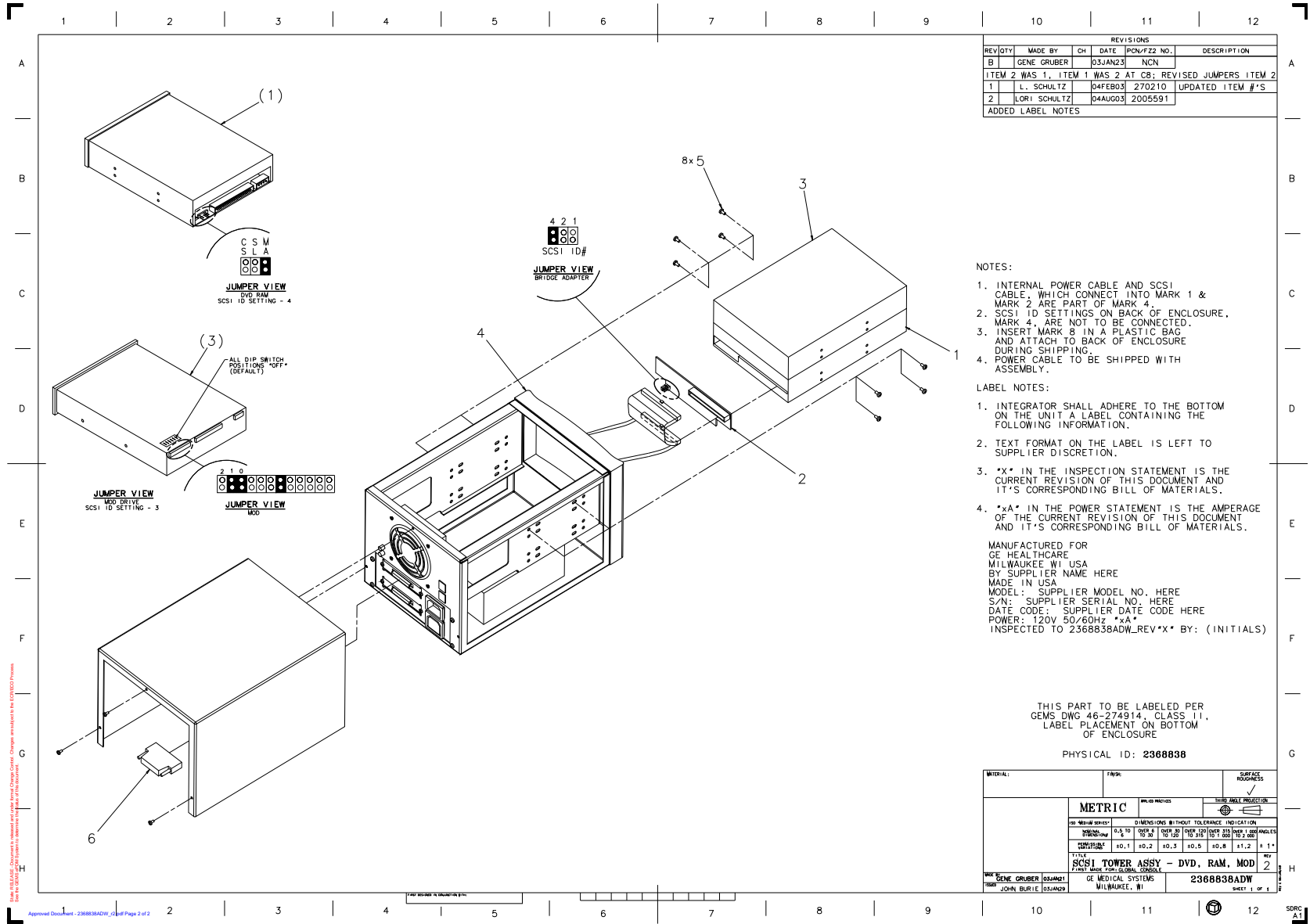
Figure 5-17 SCSI Tower, DVD-RAM, MOD (2368838, sheet 1, rev 2)
